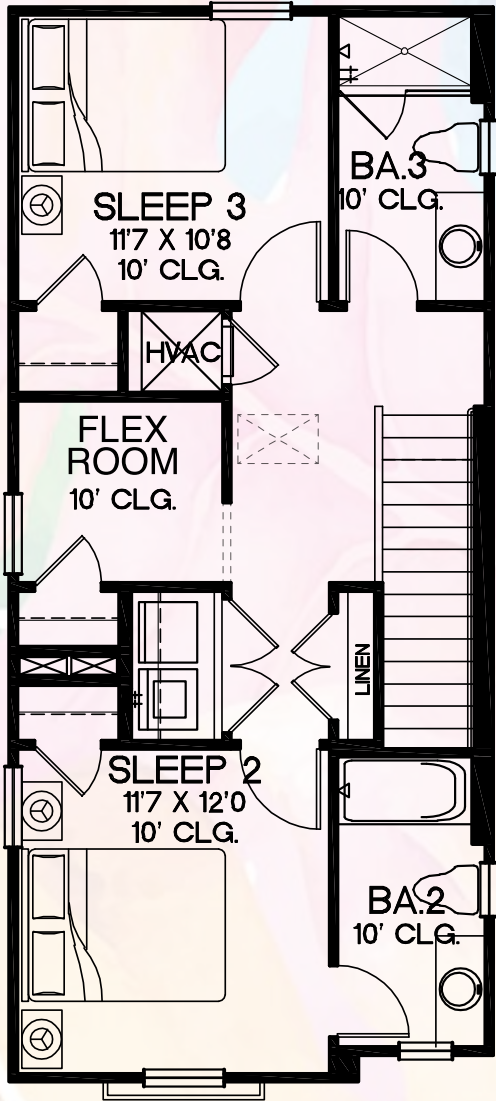
2ND FLOOR
